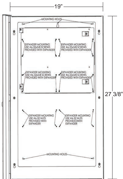
AE-14 Cabinet Dimensions
