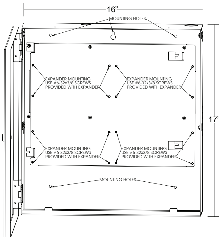
AE-8 Cabinet Dimensions
