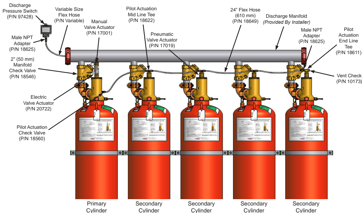
Typical Primary and Secondary Cylinder Arrangement
